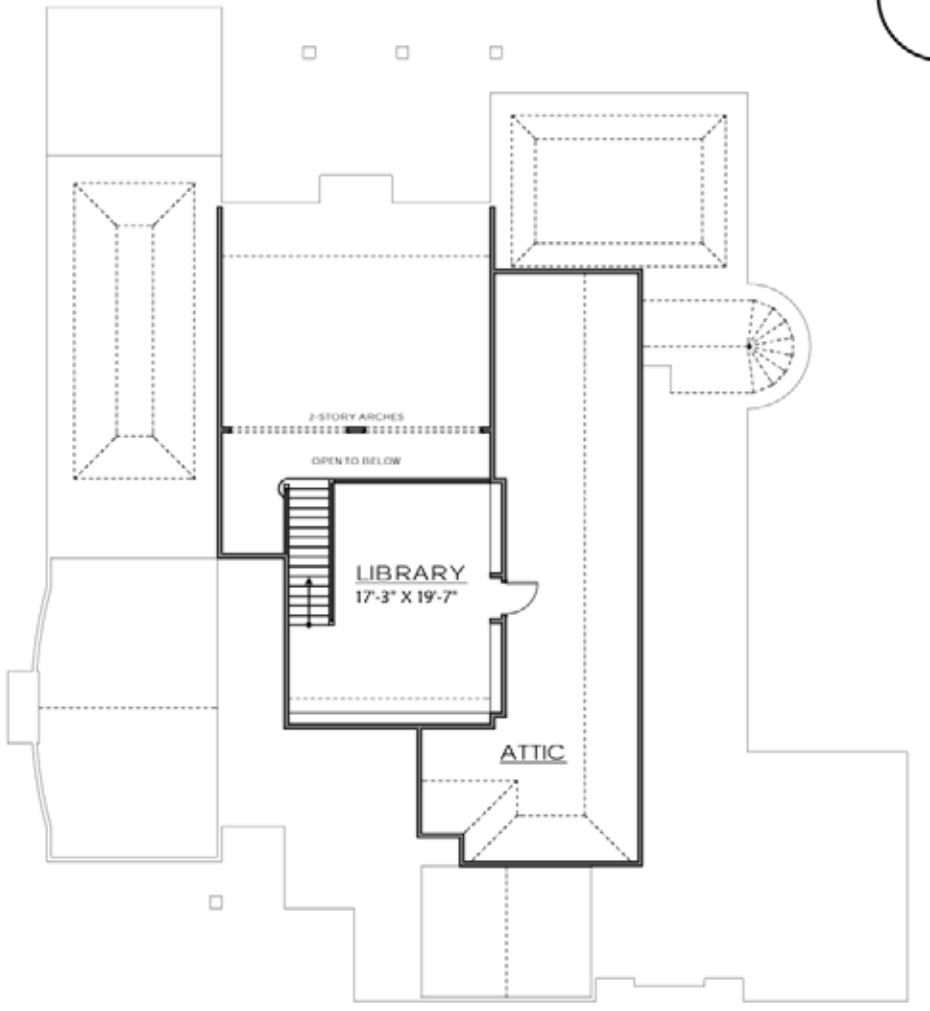
UPPER LEVEL PLAN
