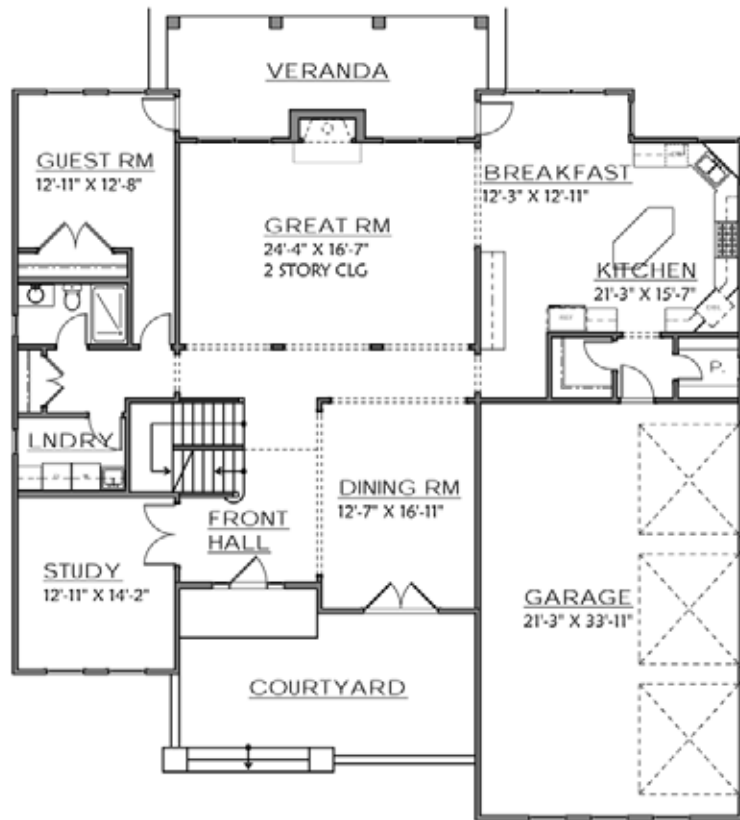
MAIN LEVEL PLAN
