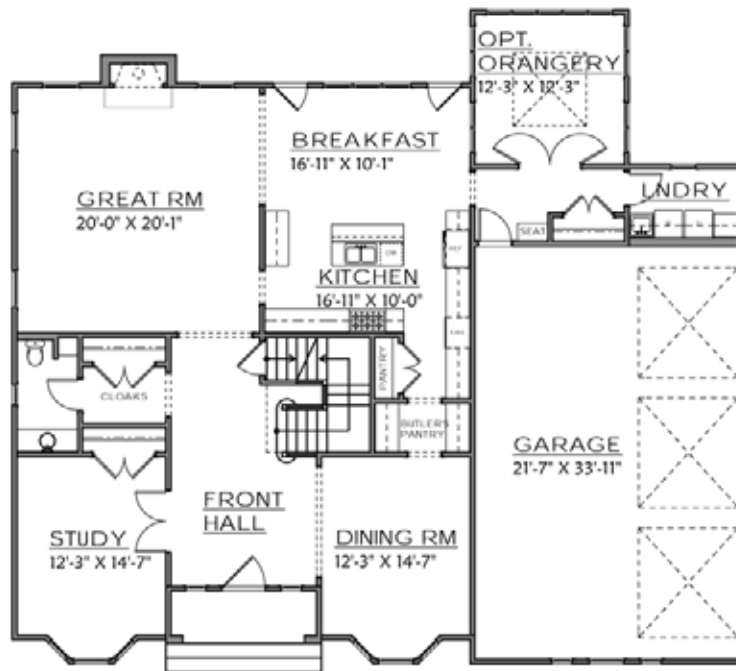
MAIN LEVEL PLAN
